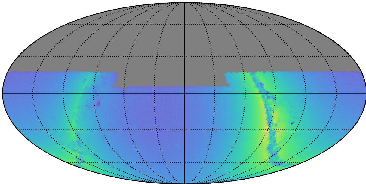
baseline_v2.0_10yrs u: Nstars_no_crowding
