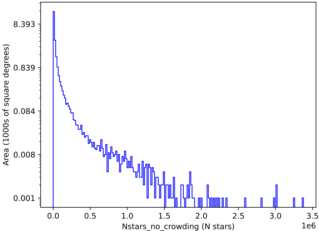
baseline_v2.0_10yrs u: Nstars_no_crowding
