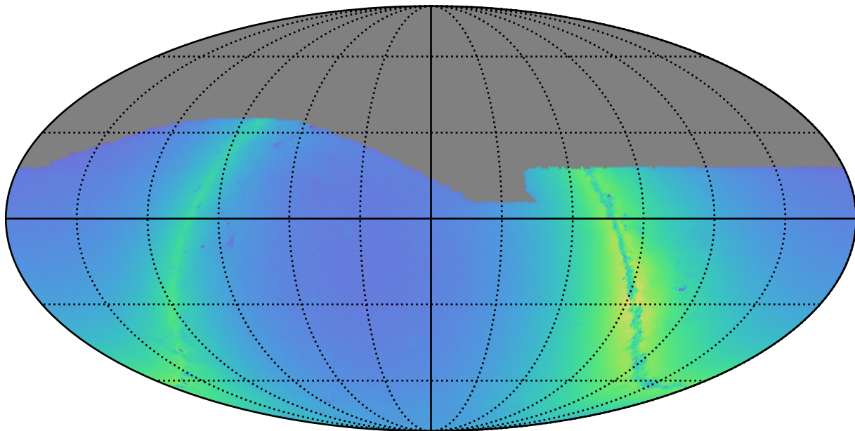
baseline_v2.0_10yrs r: Nstars_no_crowding
