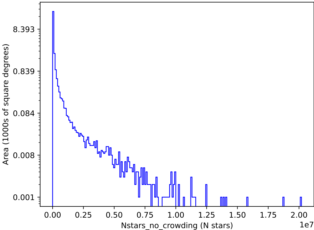
baseline_v2.0_10yrs r: Nstars_no_crowding
