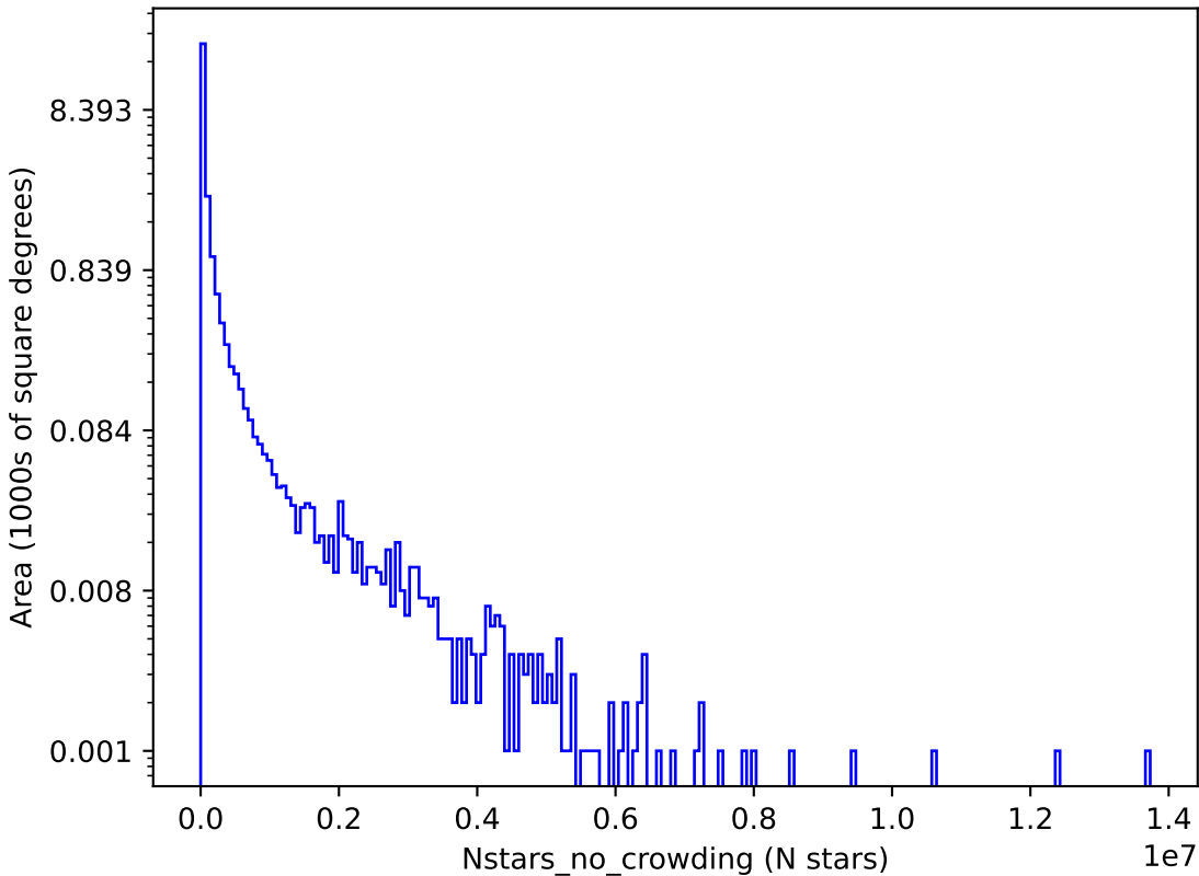
baseline_v2.0_10yrs g: Nstars_no_crowding
