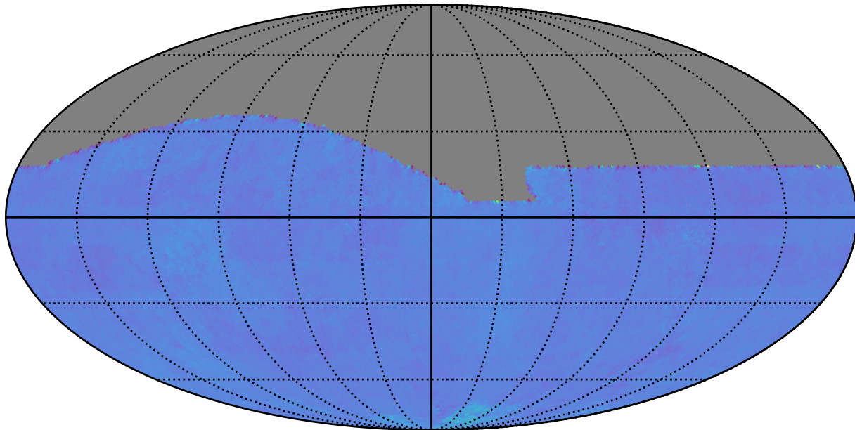
baseline_v2.0_10yrs : Normalized Proper Motion Uncert @ 24.0
