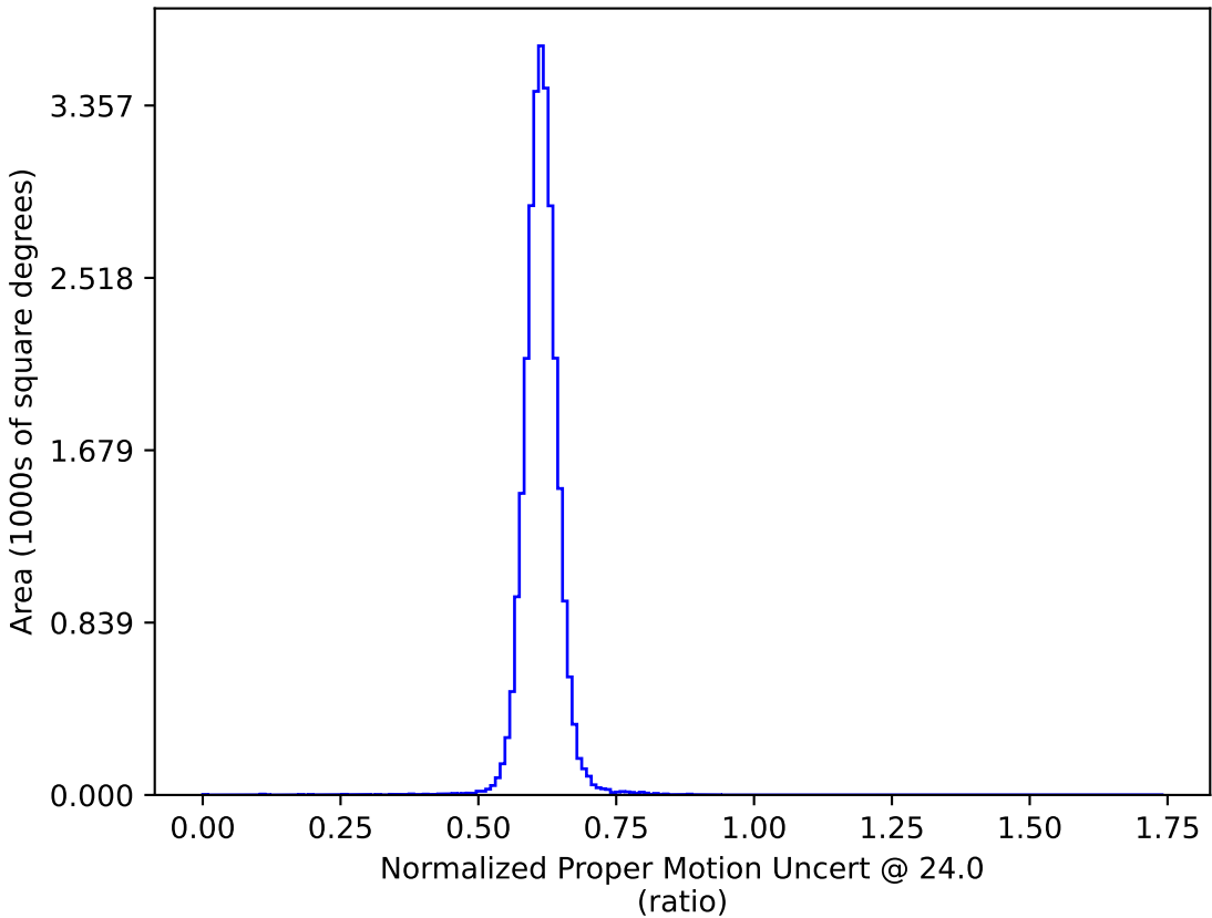
baseline_v2.0_10yrs : Normalized Proper Motion Uncert @ 24.0
