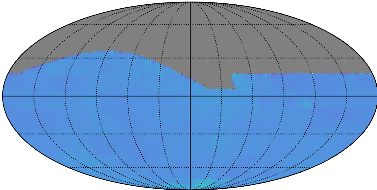
baseline_v2.0_10yrs : Normalized Proper Motion Uncert @ 20.5
