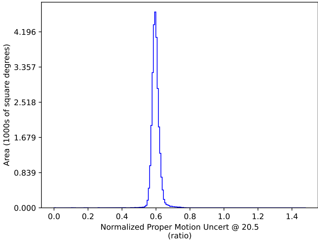
baseline_v2.0_10yrs : Normalized Proper Motion Uncert @ 20.5
