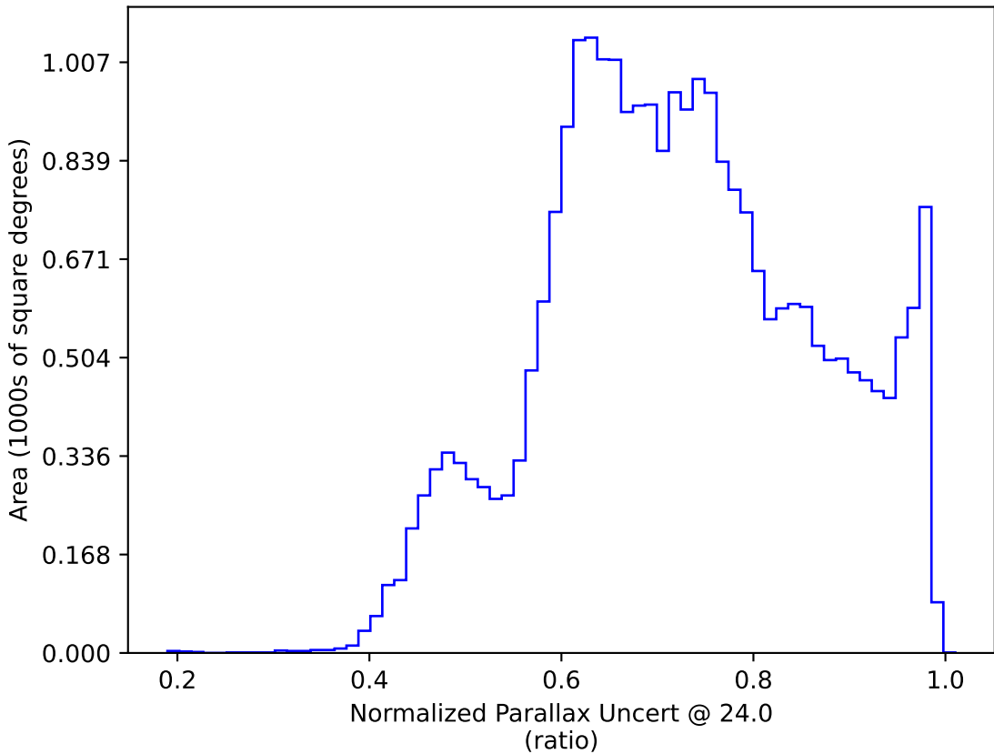
baseline_v2.0_10yrs : Normalized Parallax Uncert @ 24.0
