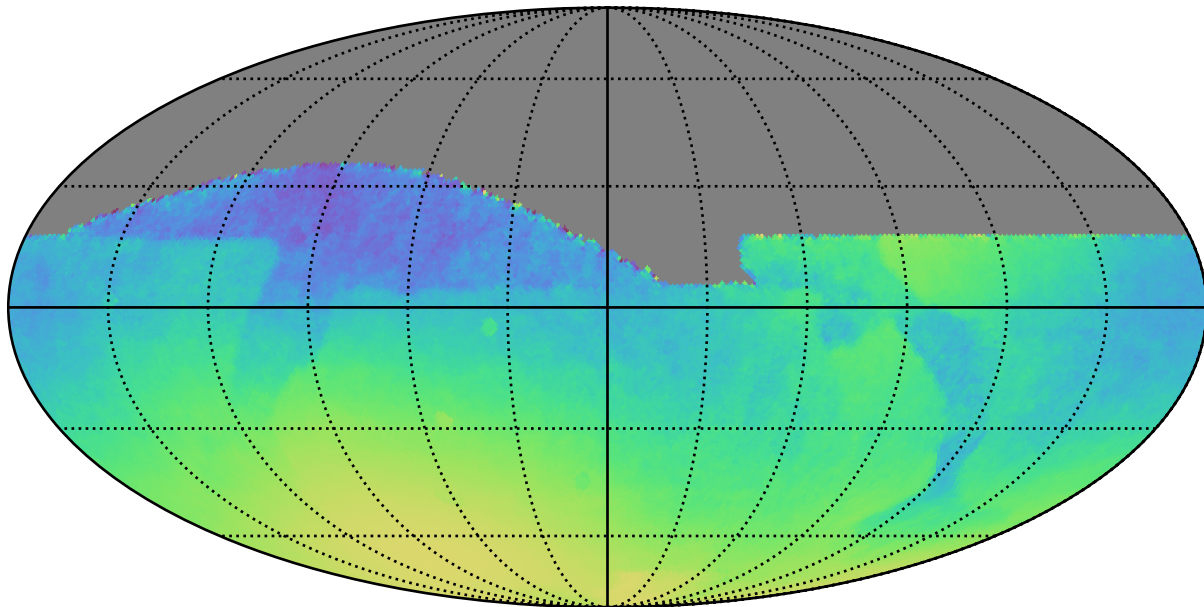
baseline_v2.0_10yrs : Normalized Parallax Uncert @ 22.4
