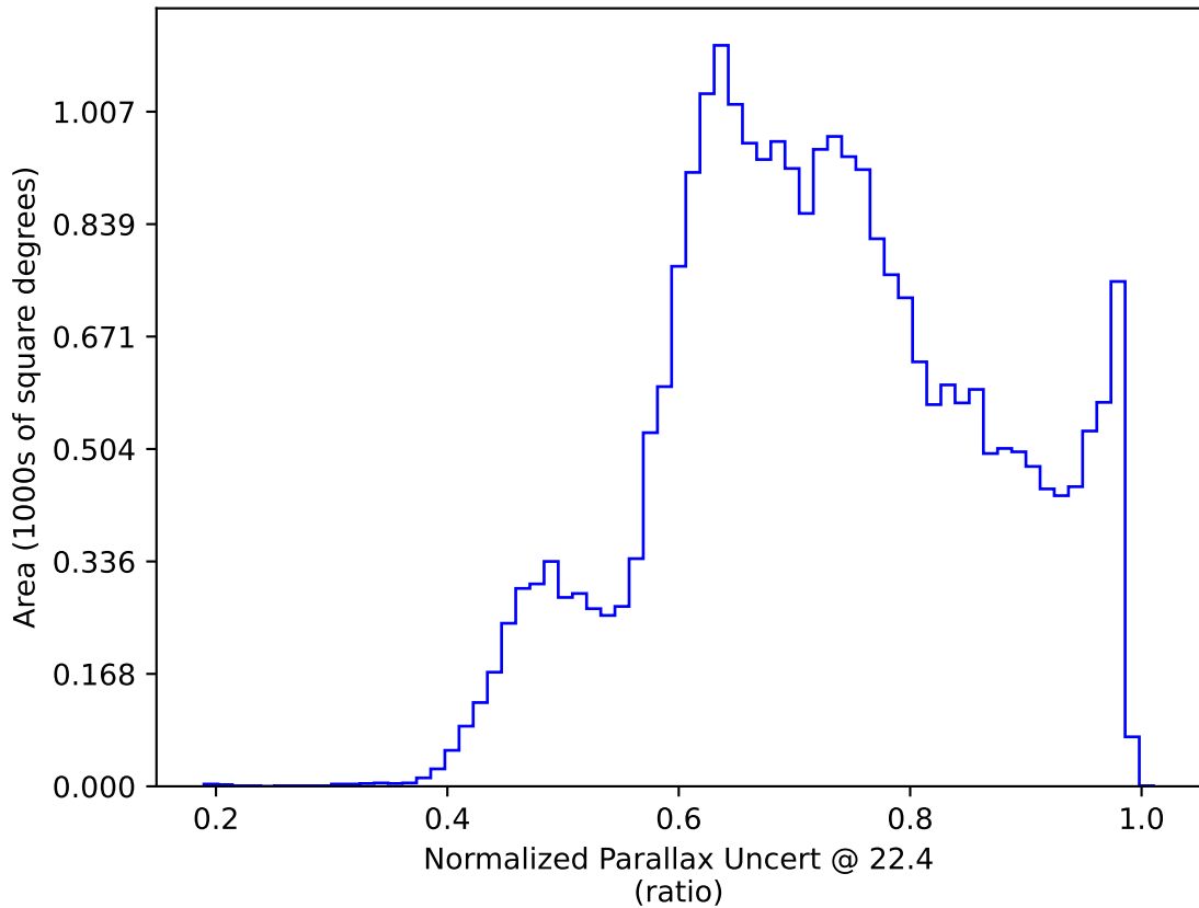
baseline_v2.0_10yrs : Normalized Parallax Uncert @ 22.4
