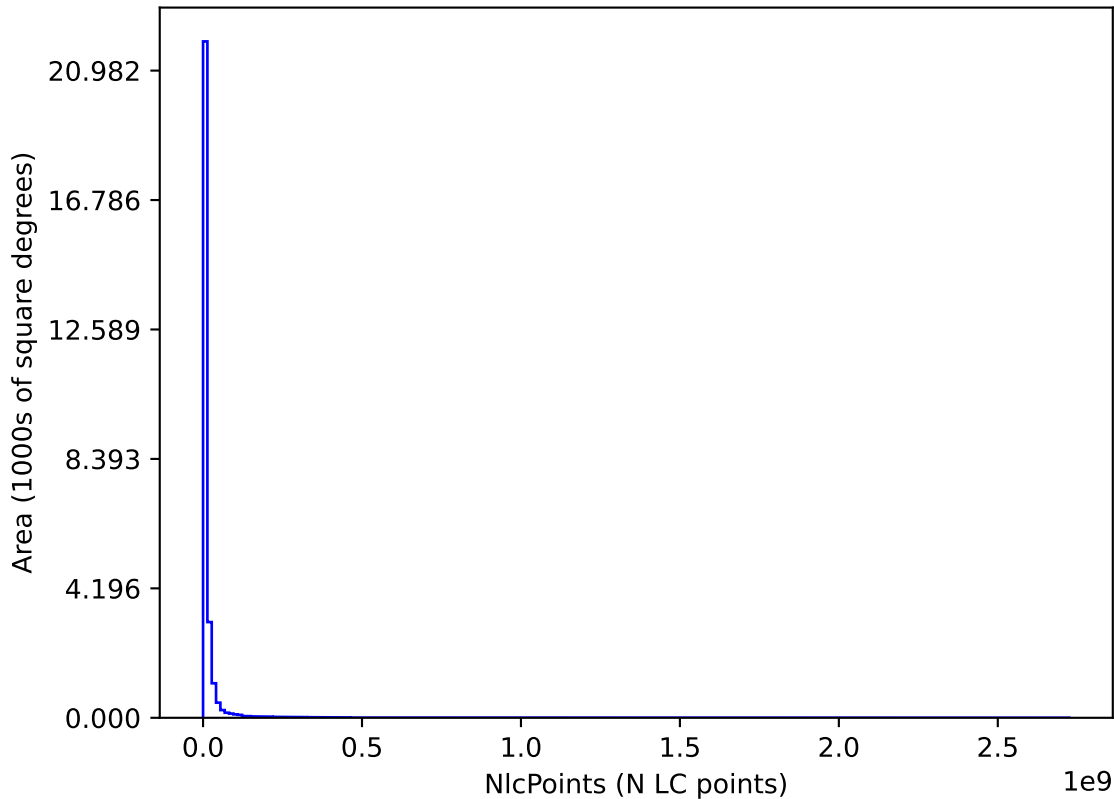
baseline_v2.0_10yrs : NlcPoints
