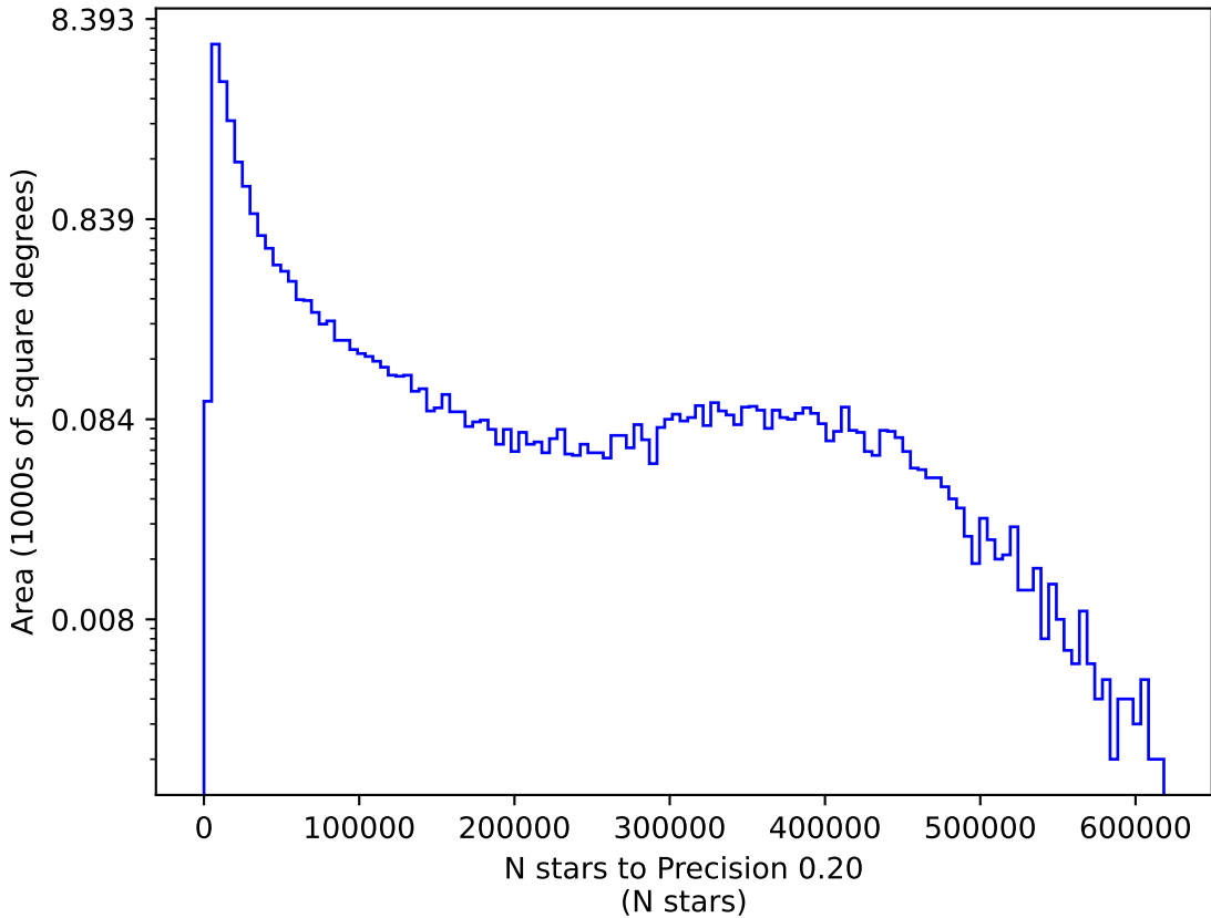
baseline_v2.0_10yrs z: N stars to Precision 0.20
