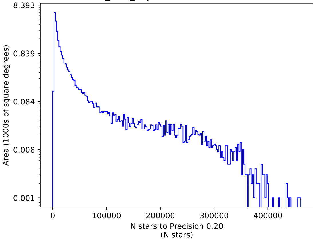
baseline_v2.0_10yrs u: N stars to Precision 0.20
