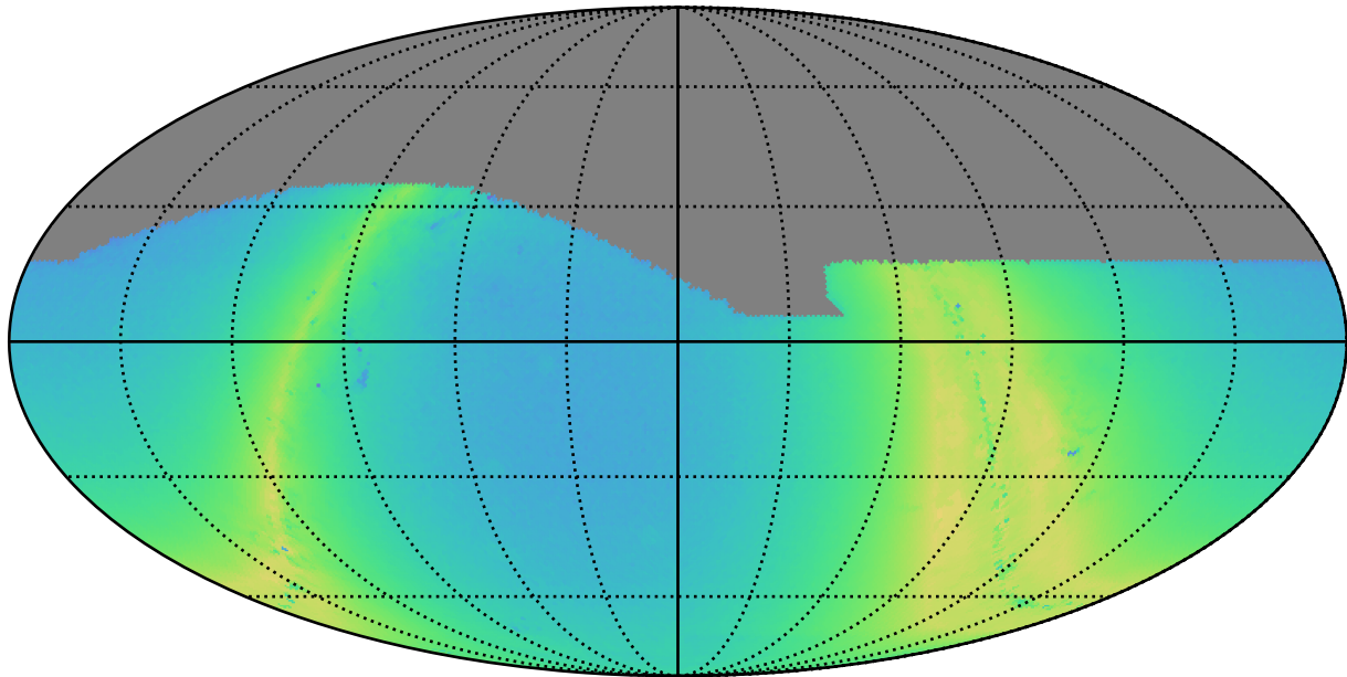
baseline_v2.0_10yrs r: N stars to Precision 0.20
