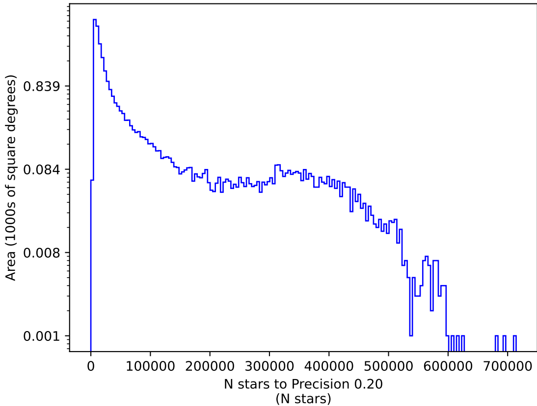
baseline_v2.0_10yrs r: N stars to Precision 0.20
