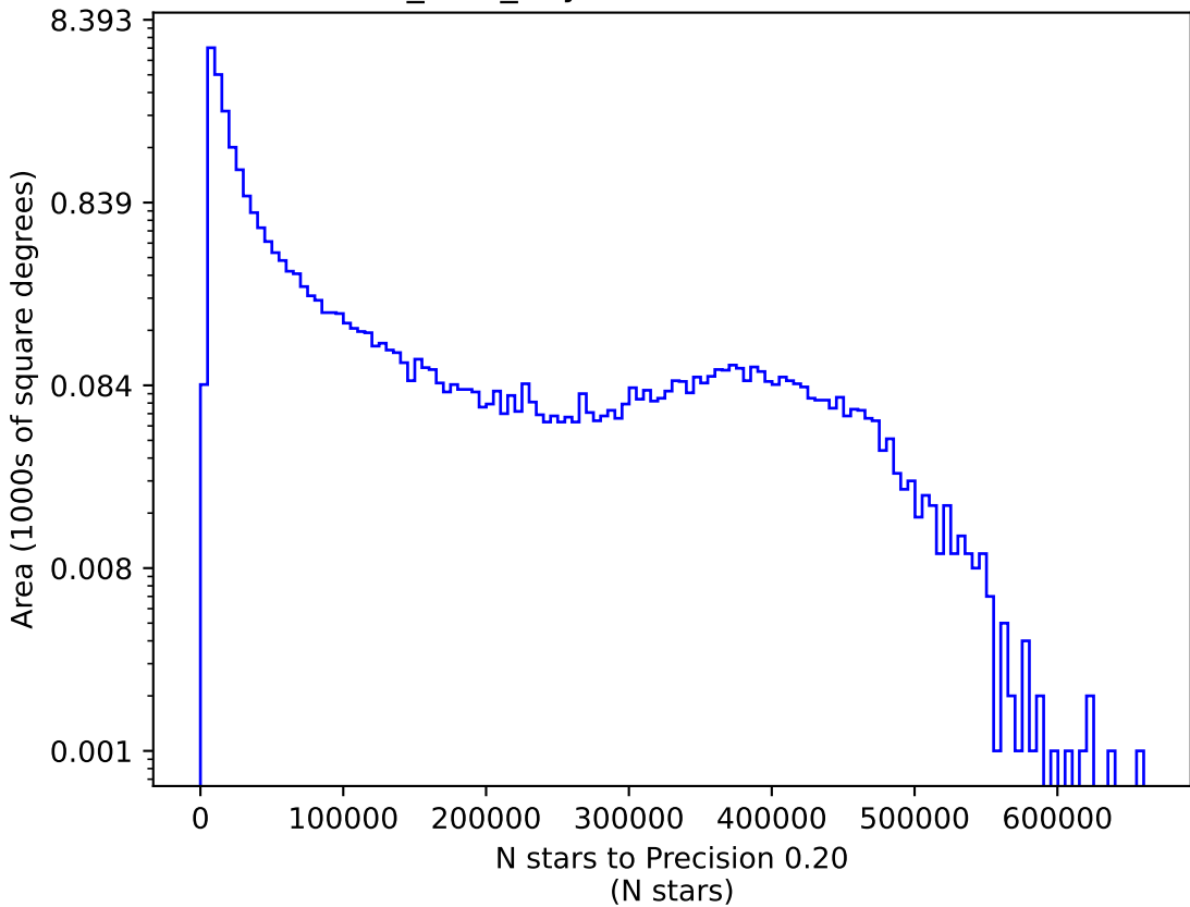
baseline_v2.0_10yrs i: N stars to Precision 0.20
