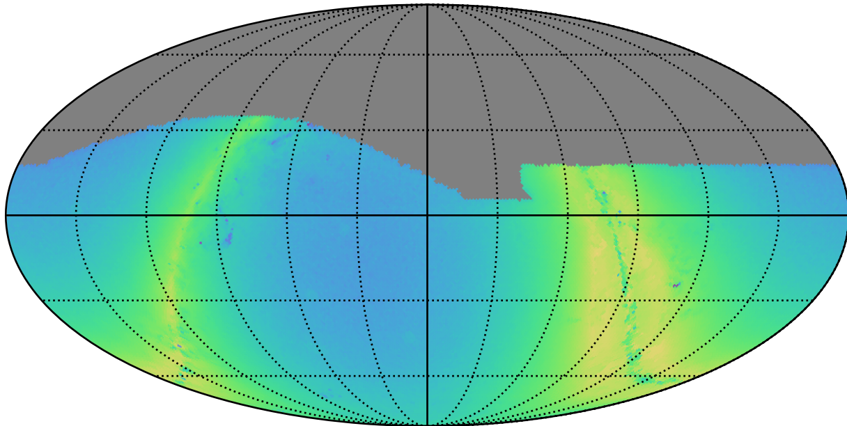
baseline_v2.0_10yrs g: N stars to Precision 0.20
