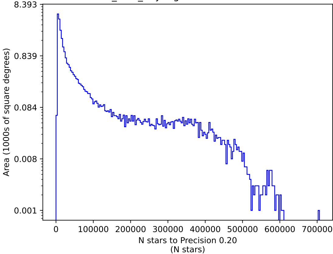
baseline_v2.0_10yrs g: N stars to Precision 0.20
