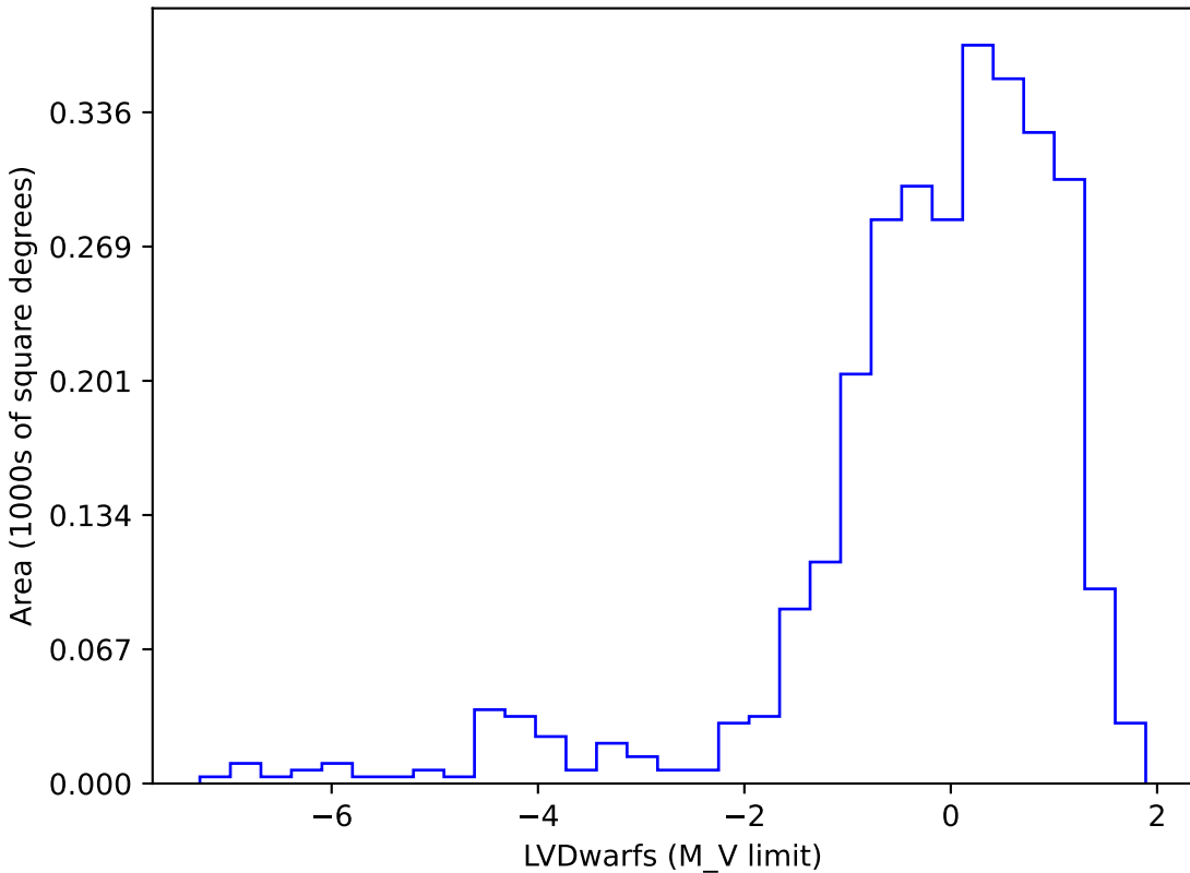
baseline_v2.0_10yrs gi SCP: LVDwarfs
