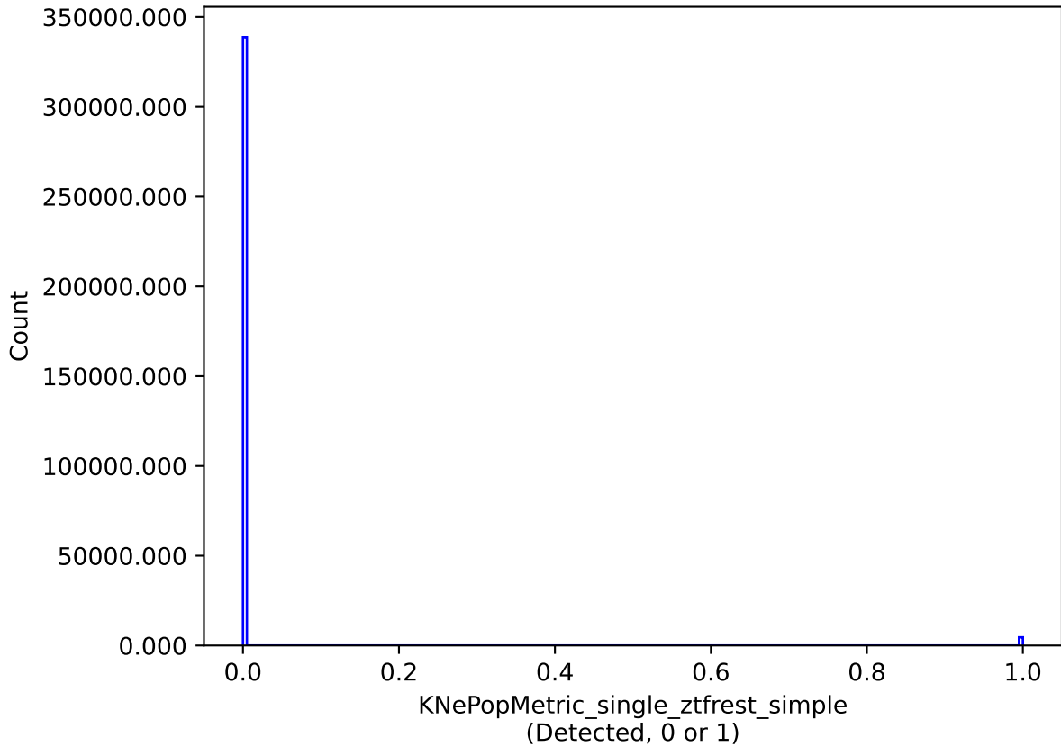
baseline_v2.0_10yrs single model: KNePopMetric_single_ztfrest_simple
