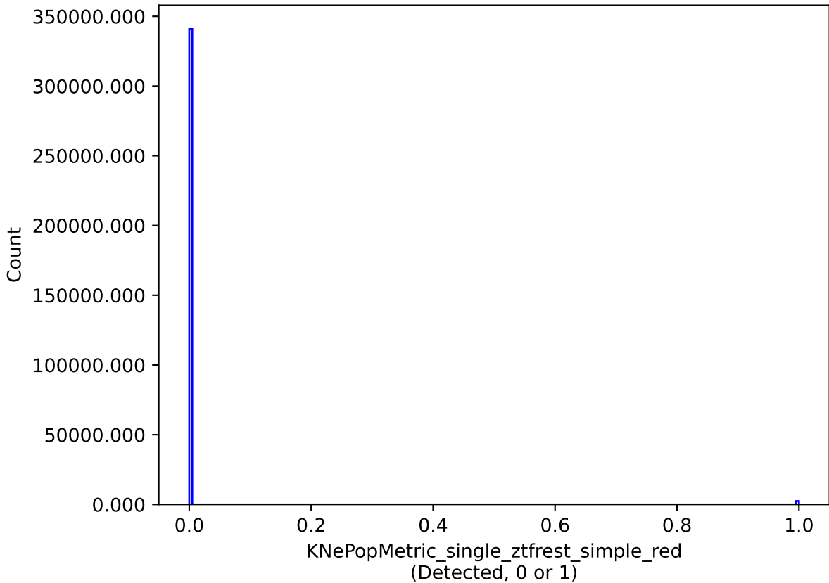
baseline_v2.0_10yrs single model: KNePopMetric_single_ztfrest_simple_red
