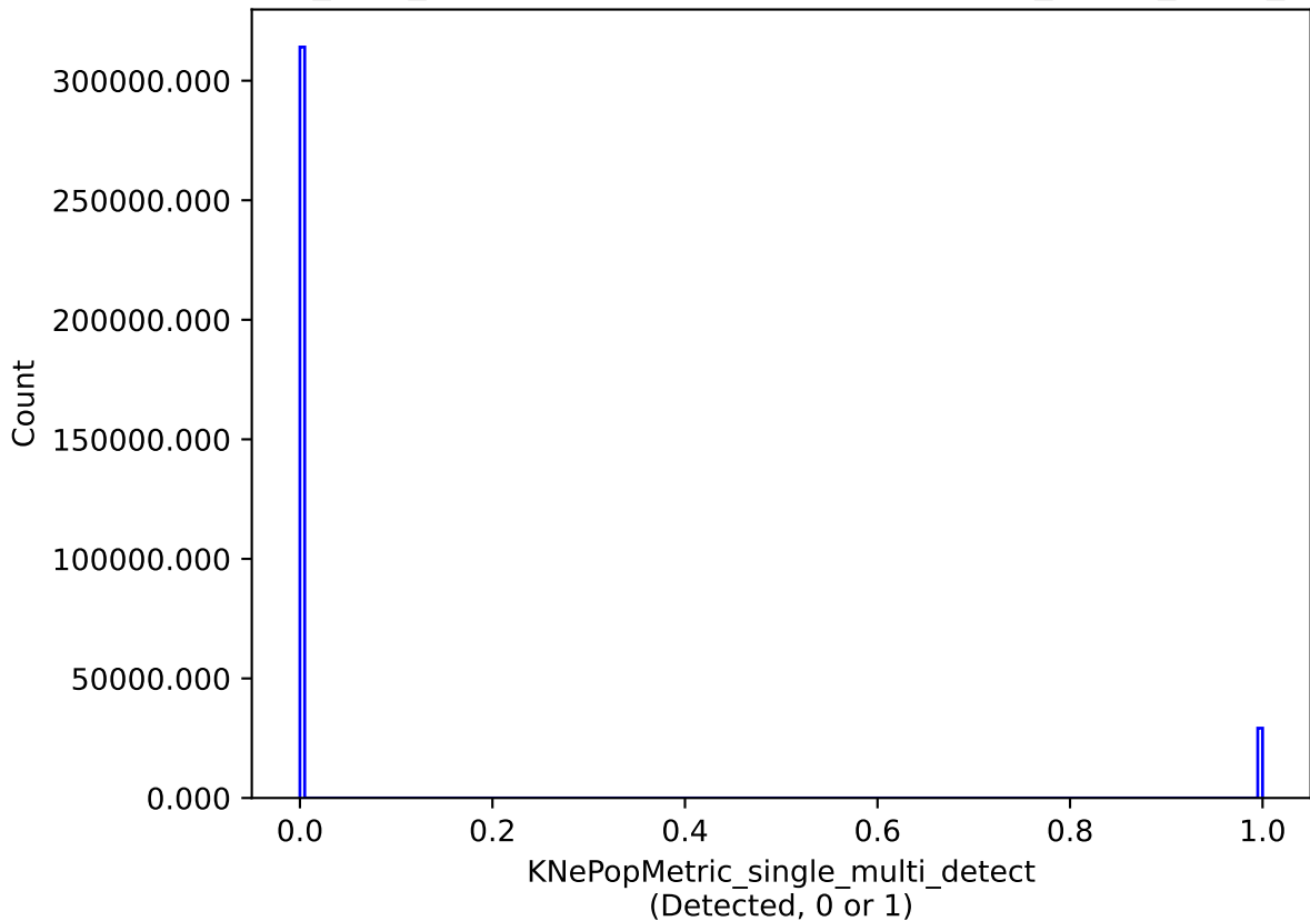
baseline_v2.0_10yrs single model: KNePopMetric_single_multi_detect
