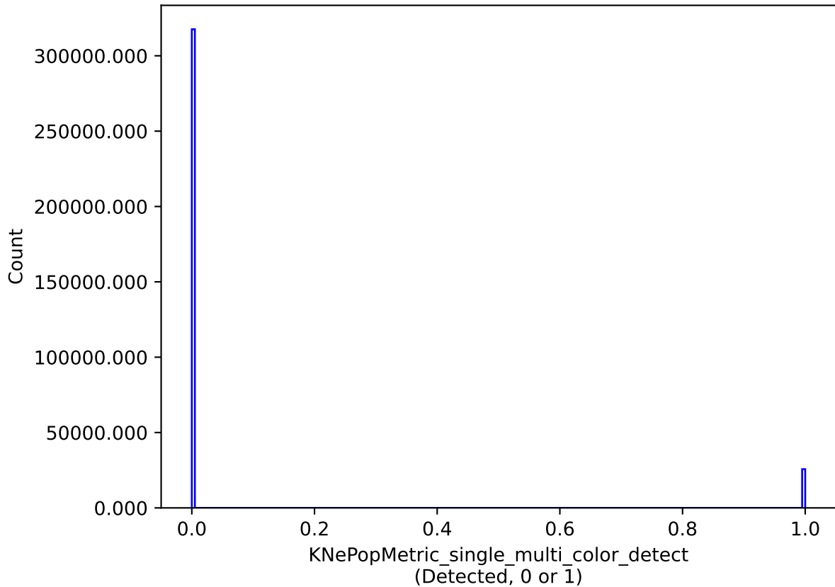
baseline_v2.0_10yrs single model: KNePopMetric_single_multi_color_detect
