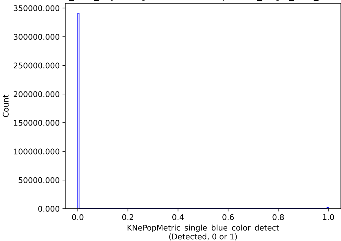
baseline_v2.0_10yrs single model: KNePopMetric_single_blue_color_detect
