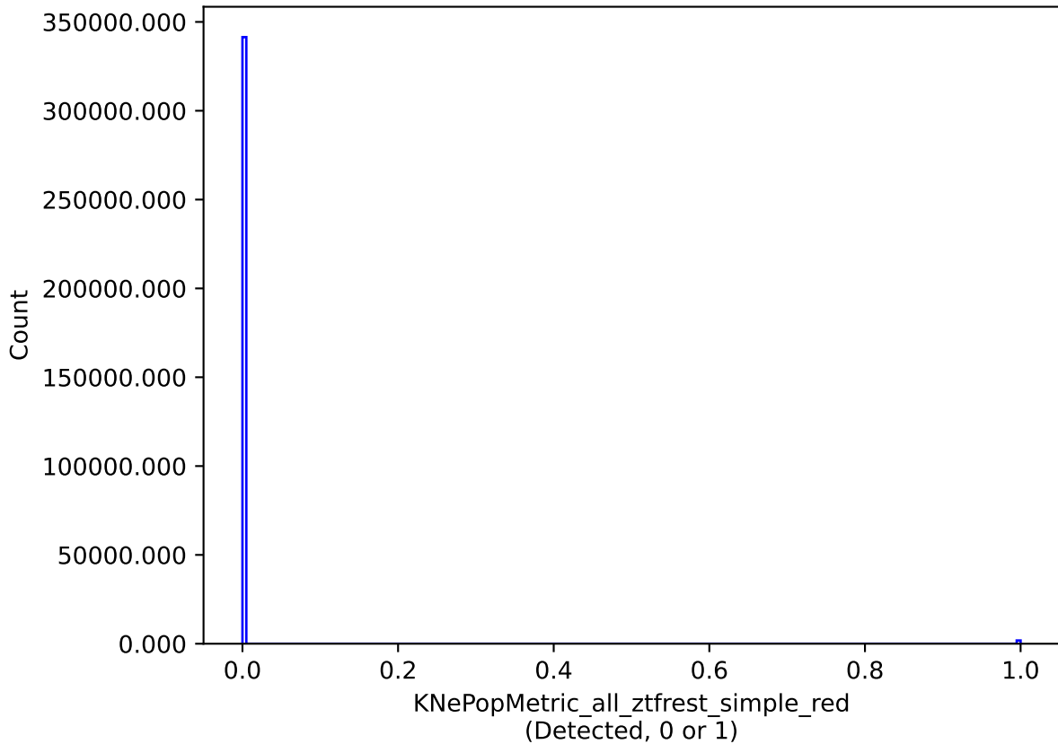
baseline_v2.0_10yrs all models: KNePopMetric_all_ztfrest_simple_red
