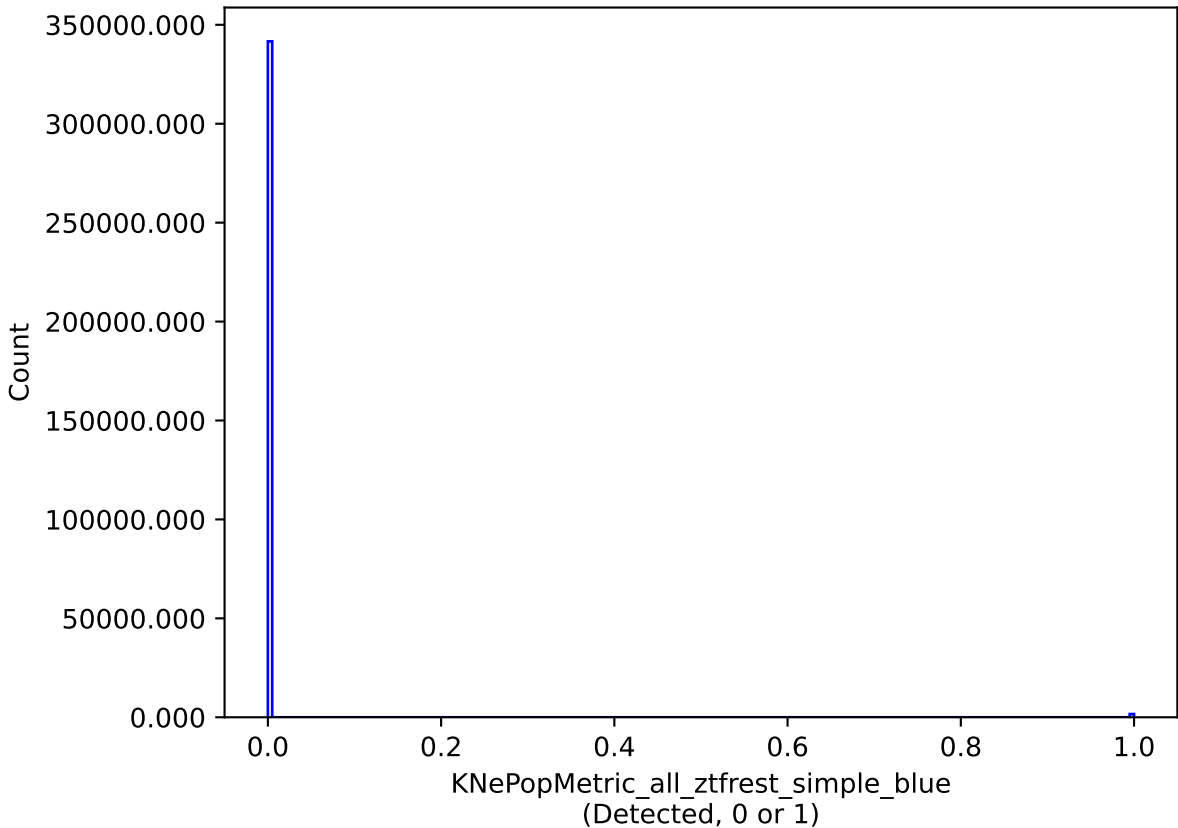
baseline_v2.0_10yrs all models: KNePopMetric_all_ztfrest_simple_blue
