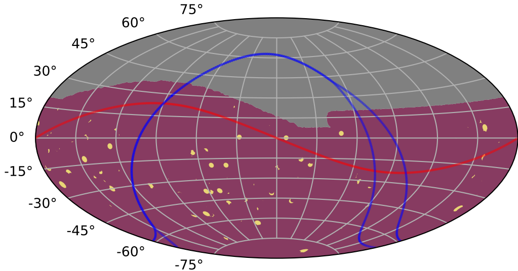
baseline_v2.0_10yrs all models: KNePopMetric_all_ztfrest_simple
