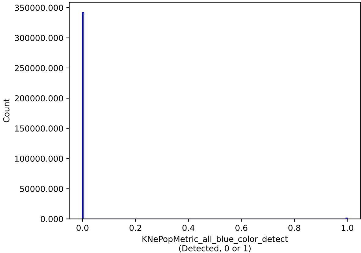
baseline_v2.0_10yrs all models: KNePopMetric_all_blue_color_detect
