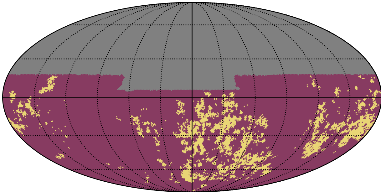
baseline_v2.0_10yrs y band: Gaps_7hr
