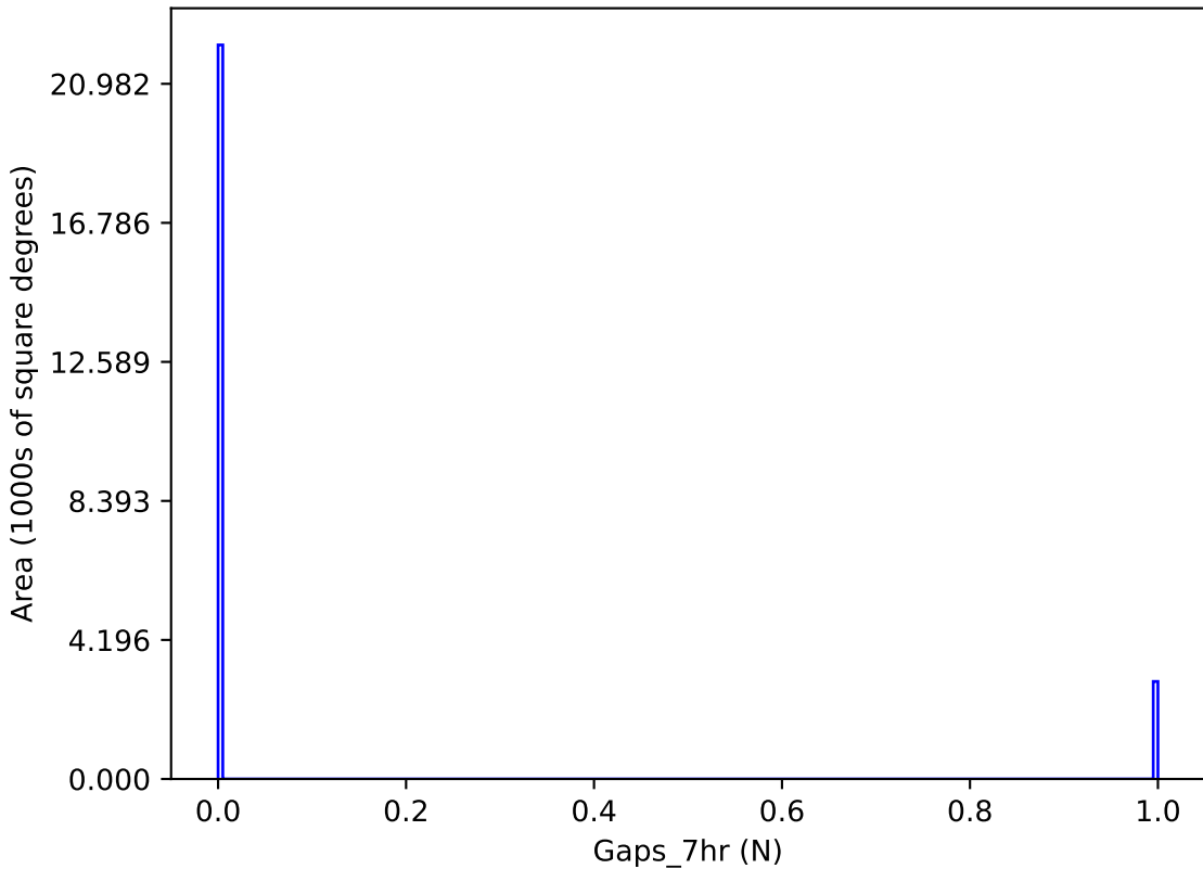
baseline_v2.0_10yrs y band: Gaps_7hr
