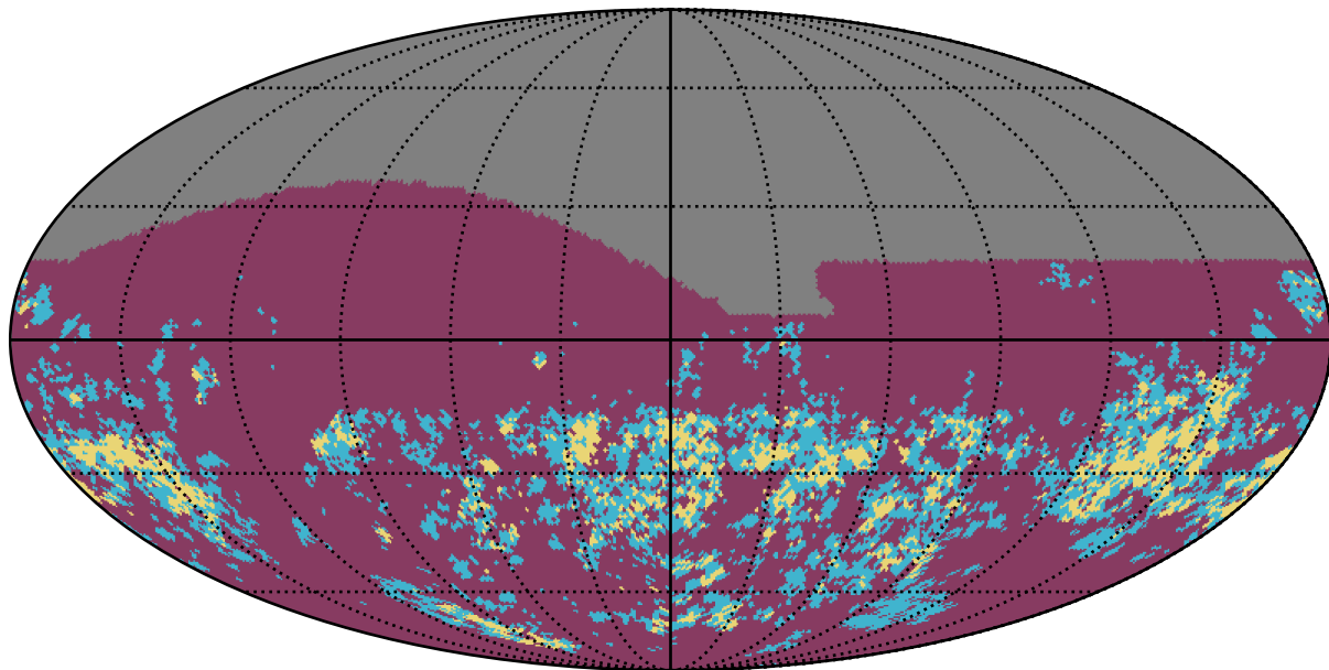
baseline_v2.0_10yrs r band: Gaps_7hr
