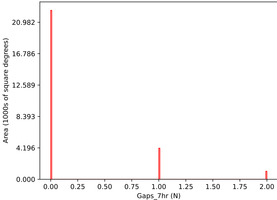
baseline_v2.0_10yrs i band: Gaps_7hr
