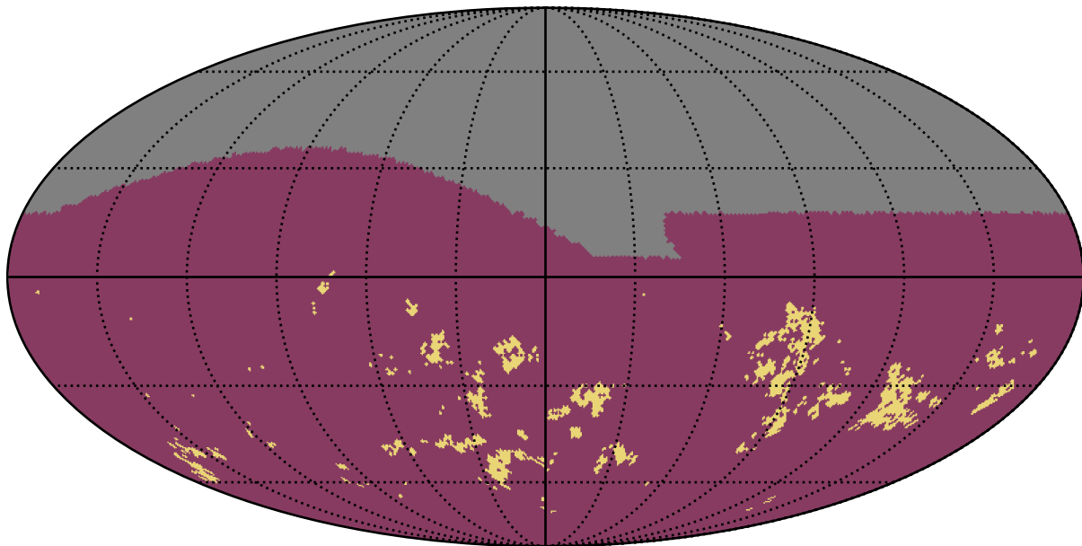
baseline_v2.0_10yrs g band: Gaps_7hr
