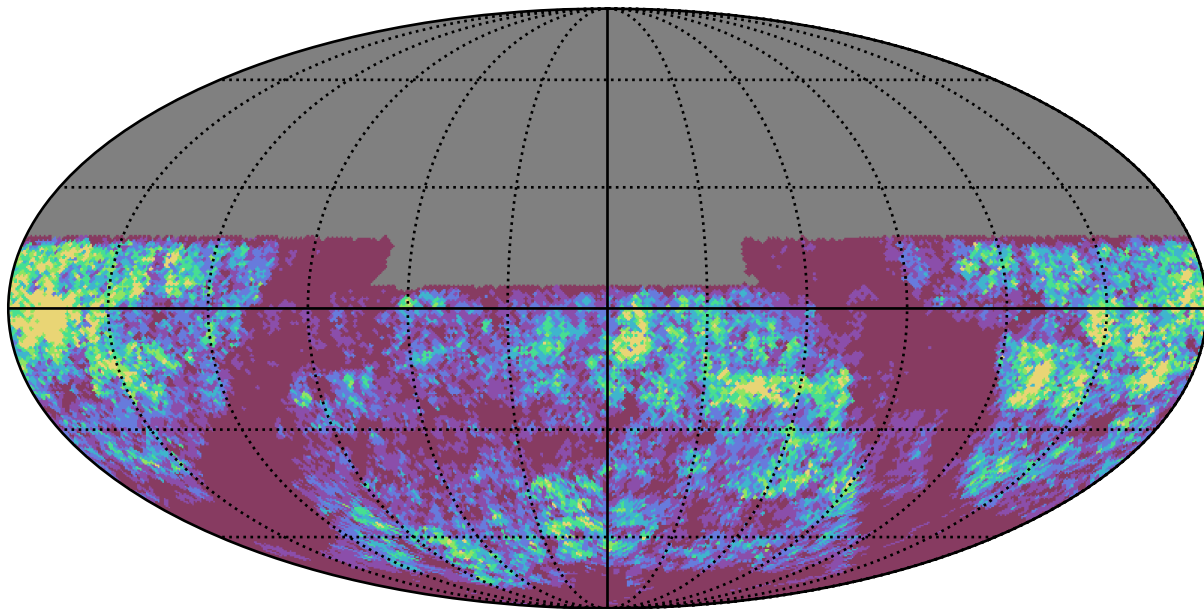
baseline_v2.0_10yrs y band: Gaps_3hr
