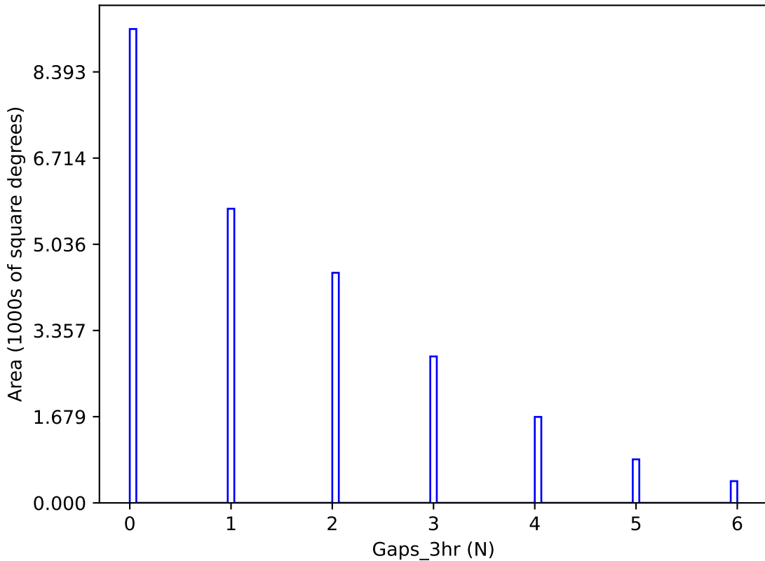
baseline_v2.0_10yrs y band: Gaps_3hr
