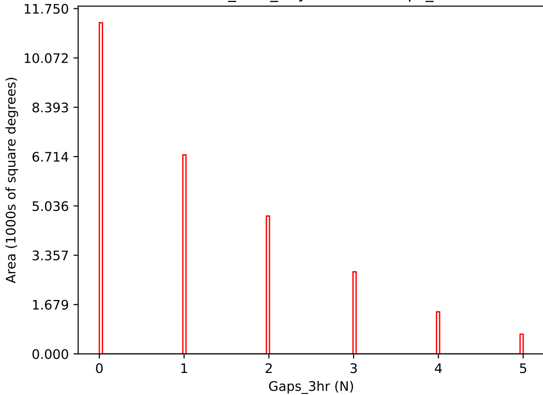
baseline_v2.0_10yrs i band: Gaps_3hr
