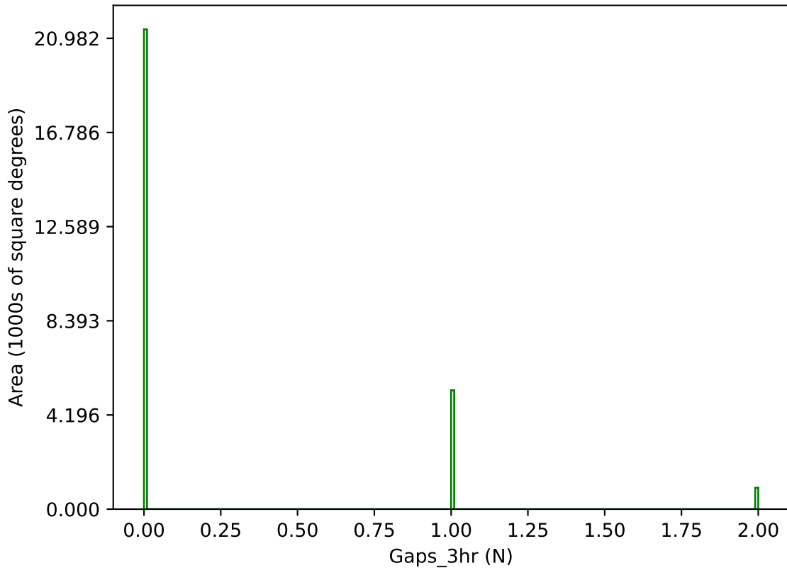
baseline_v2.0_10yrs g band: Gaps_3hr
