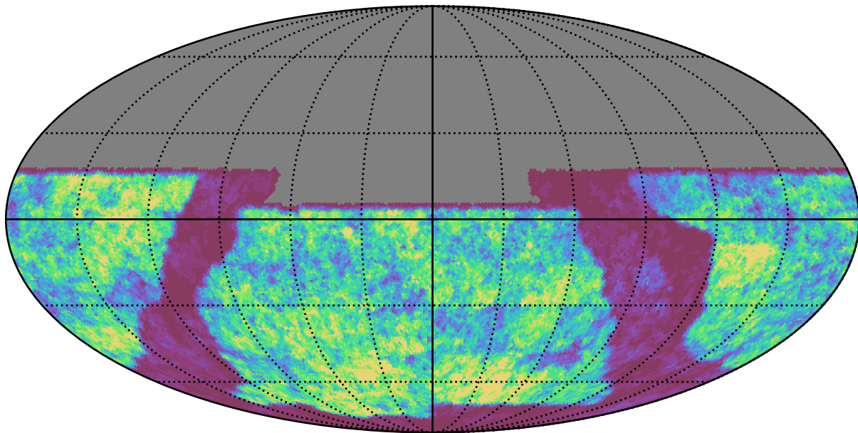
baseline_v2.0_10yrs y band: Gaps_24hr
