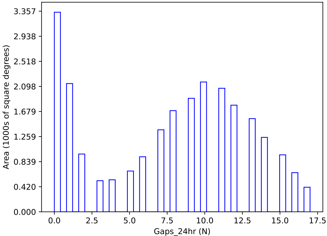
baseline_v2.0_10yrs y band: Gaps_24hr
