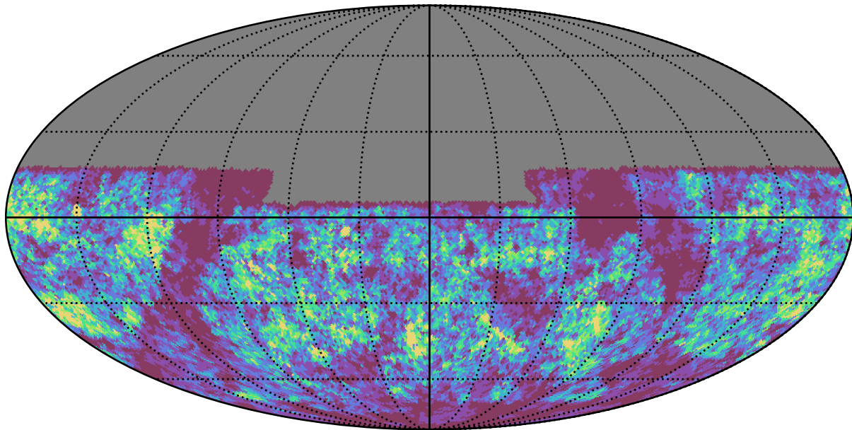
baseline_v2.0_10yrs u band: Gaps_24hr
