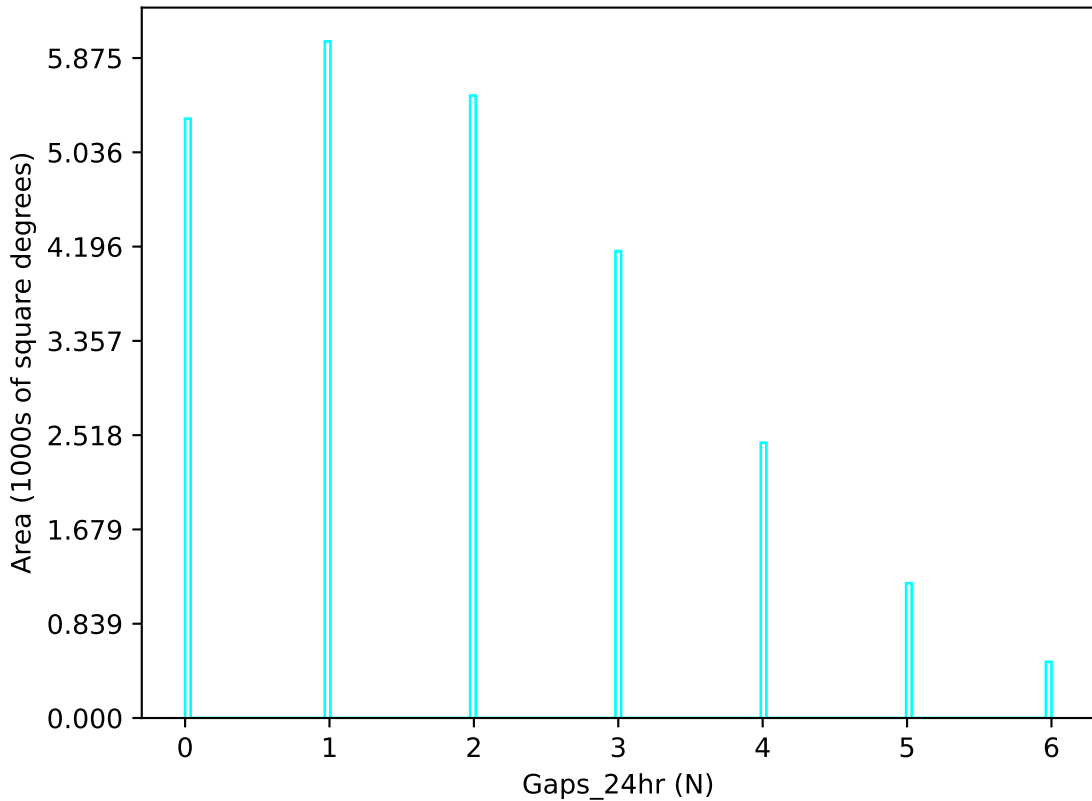
baseline_v2.0_10yrs u band: Gaps_24hr
