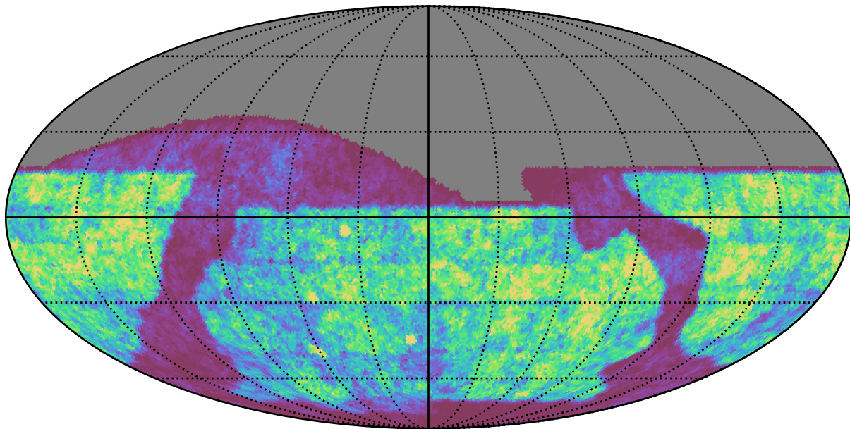
baseline_v2.0_10yrs i band: Gaps_24hr
