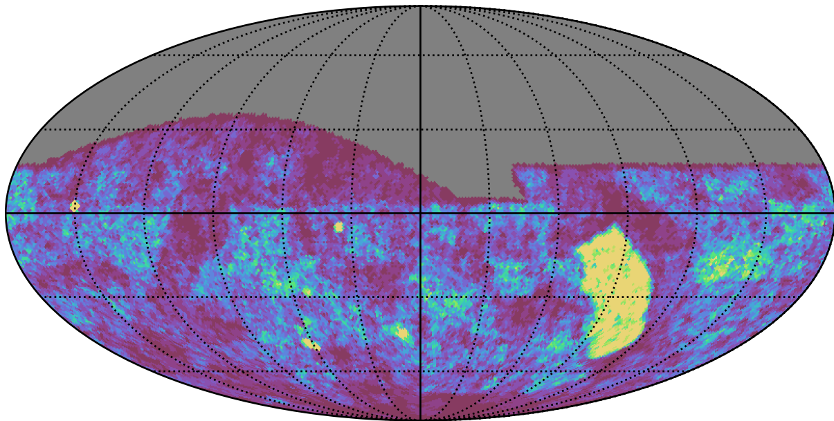
baseline_v2.0_10yrs g band: Gaps_24hr
