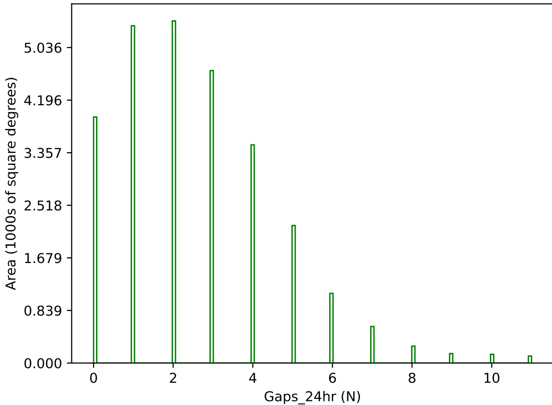
baseline_v2.0_10yrs g band: Gaps_24hr
