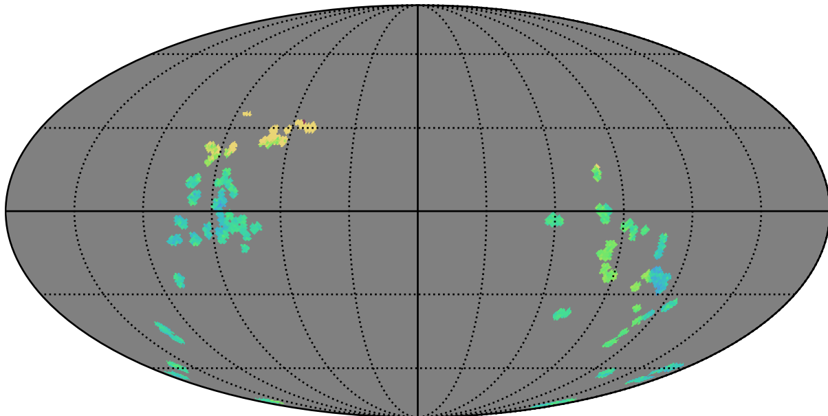
baseline_v2.0_10yrs : GalplaneTimePerFilter_zucker_sfr_map_z
