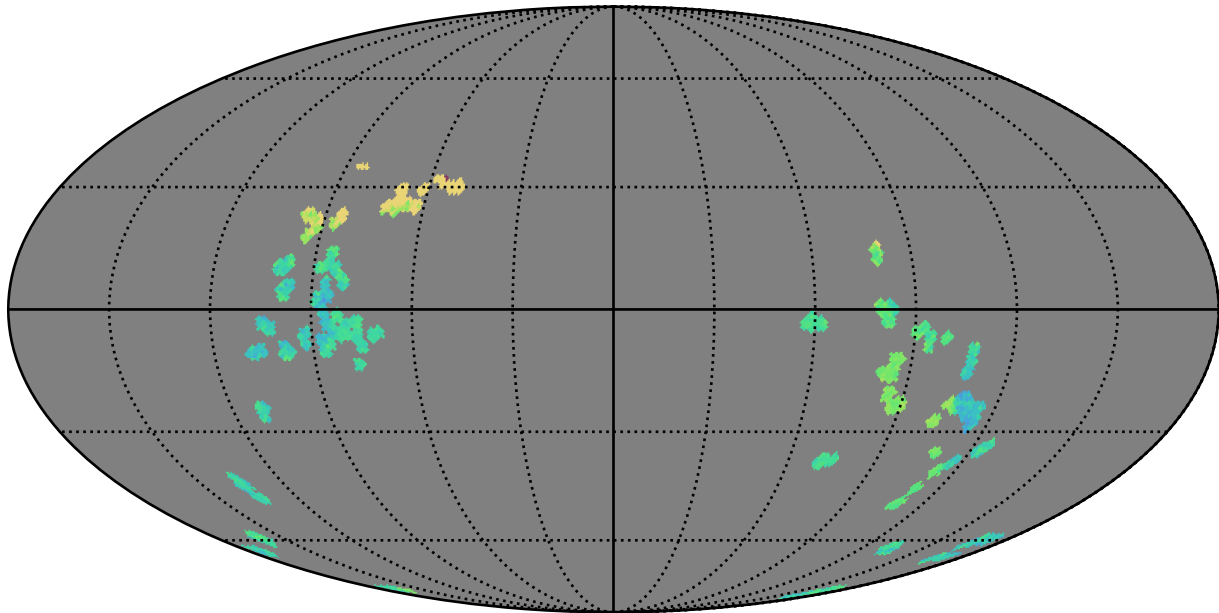
baseline_v2.0_10yrs : GalplaneTimePerFilter_zucker_sfr_map_z
