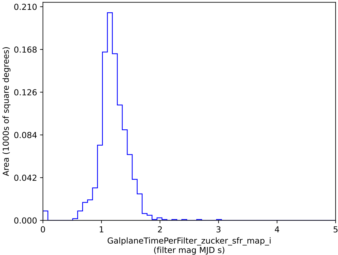
baseline_v2.0_10yrs : GalplaneTimePerFilter_zucker_sfr_map_i
