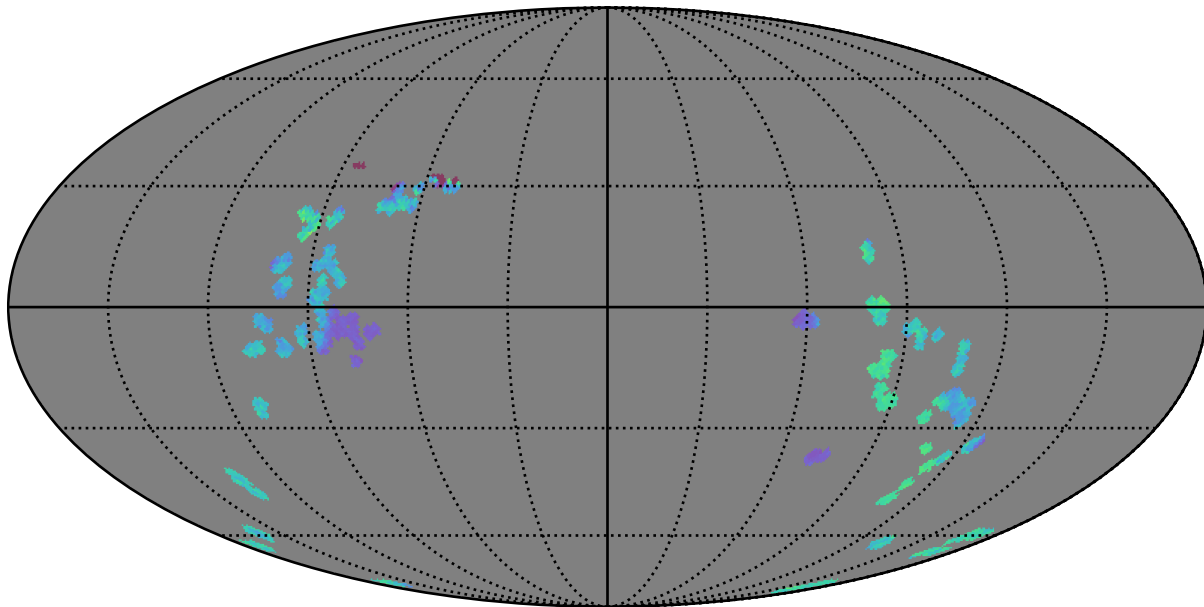
baseline_v2.0_10yrs : GalplaneTimePerFilter_zucker_sfr_map_g
