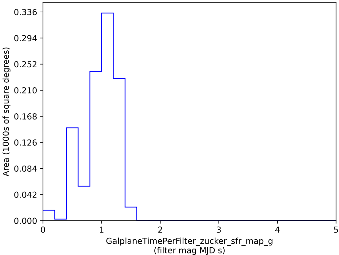
baseline_v2.0_10yrs : GalplaneTimePerFilter_zucker_sfr_map_g
